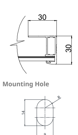
Frame Cross Section A-A
