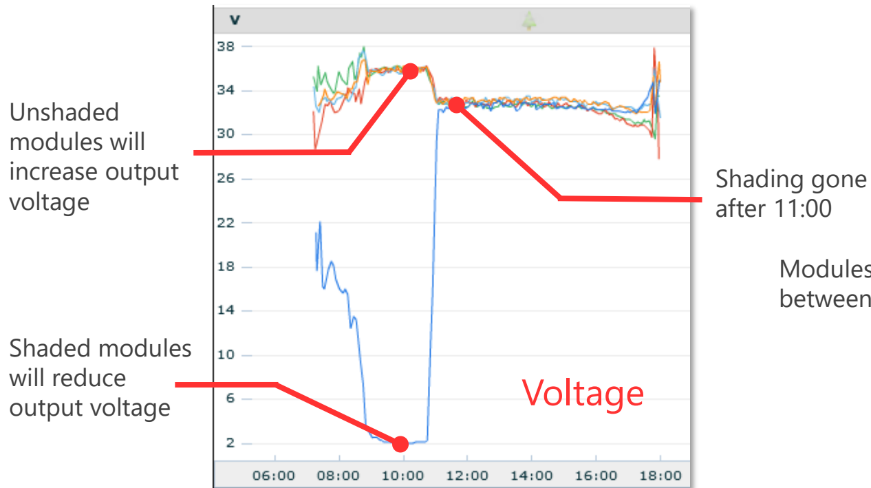
One shaded power optimizer:
