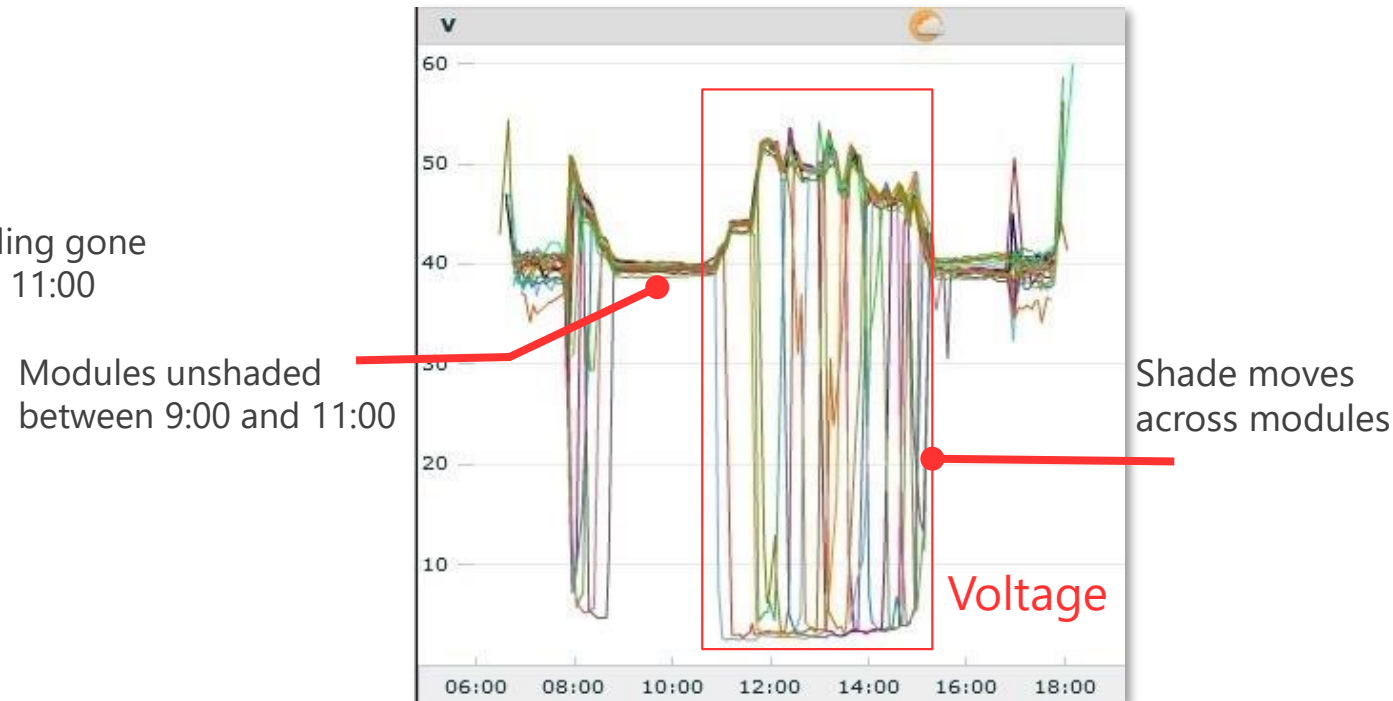
Multiple shaded power optimizers:
