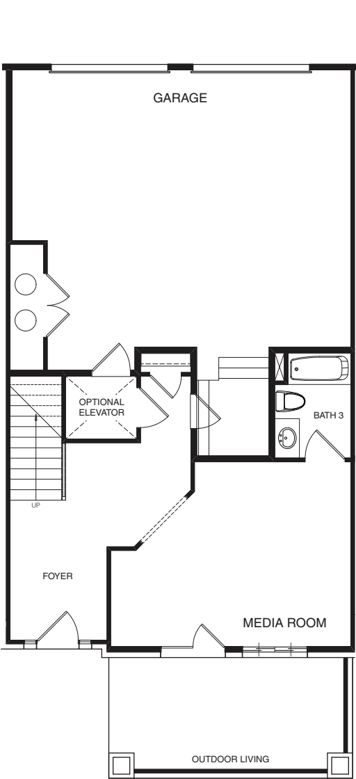
FIRST FLOOR PLAN ELEVATION A
