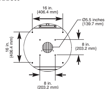
Model TBBS05
