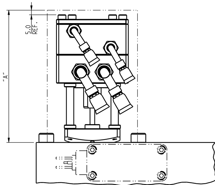
STANDARD PNEUMATIC ACTUATOR PACKAGES
