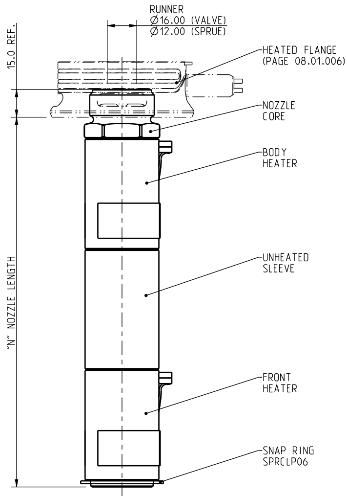
NOZZLE WITH HEATED FLANGE SHOWN
