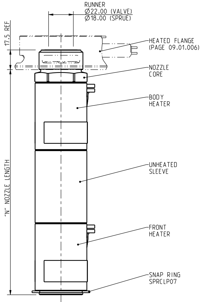
NOZZLE WITH HEATED FLANGE SHOWN
